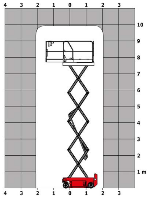
Laaddiagram
